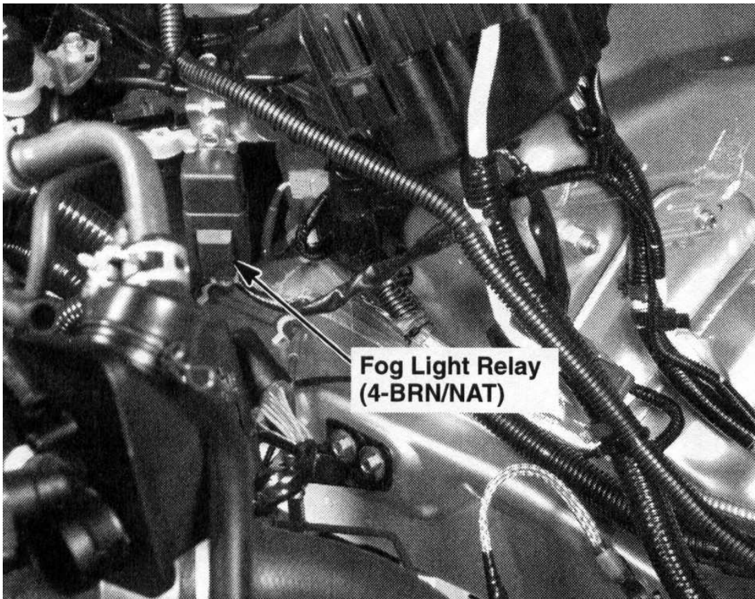
Fig. 118: Left Side Of Engine Compartment Courtesy of AMERICAN HONDA MOTOR CO., INC.
